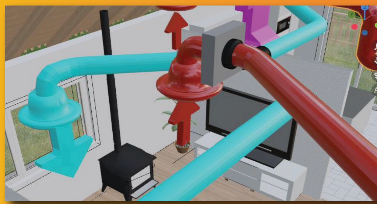
Heat Transfer System
