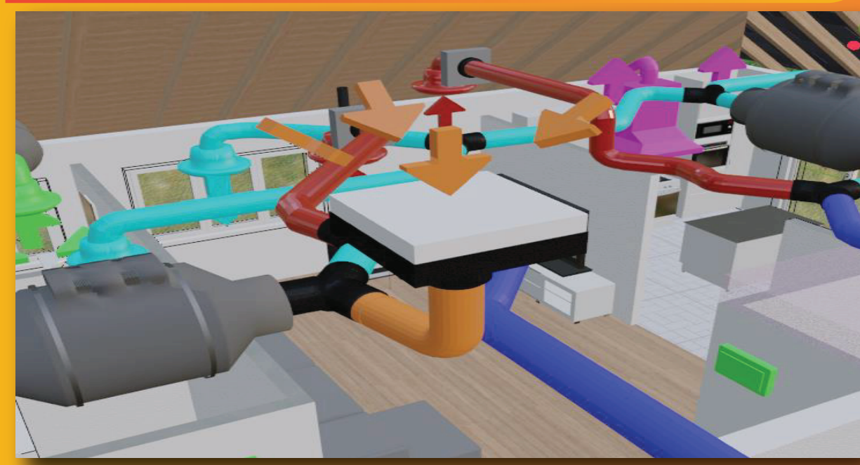
Roof Air ( Thermal Gain from the Roof Cavity )
